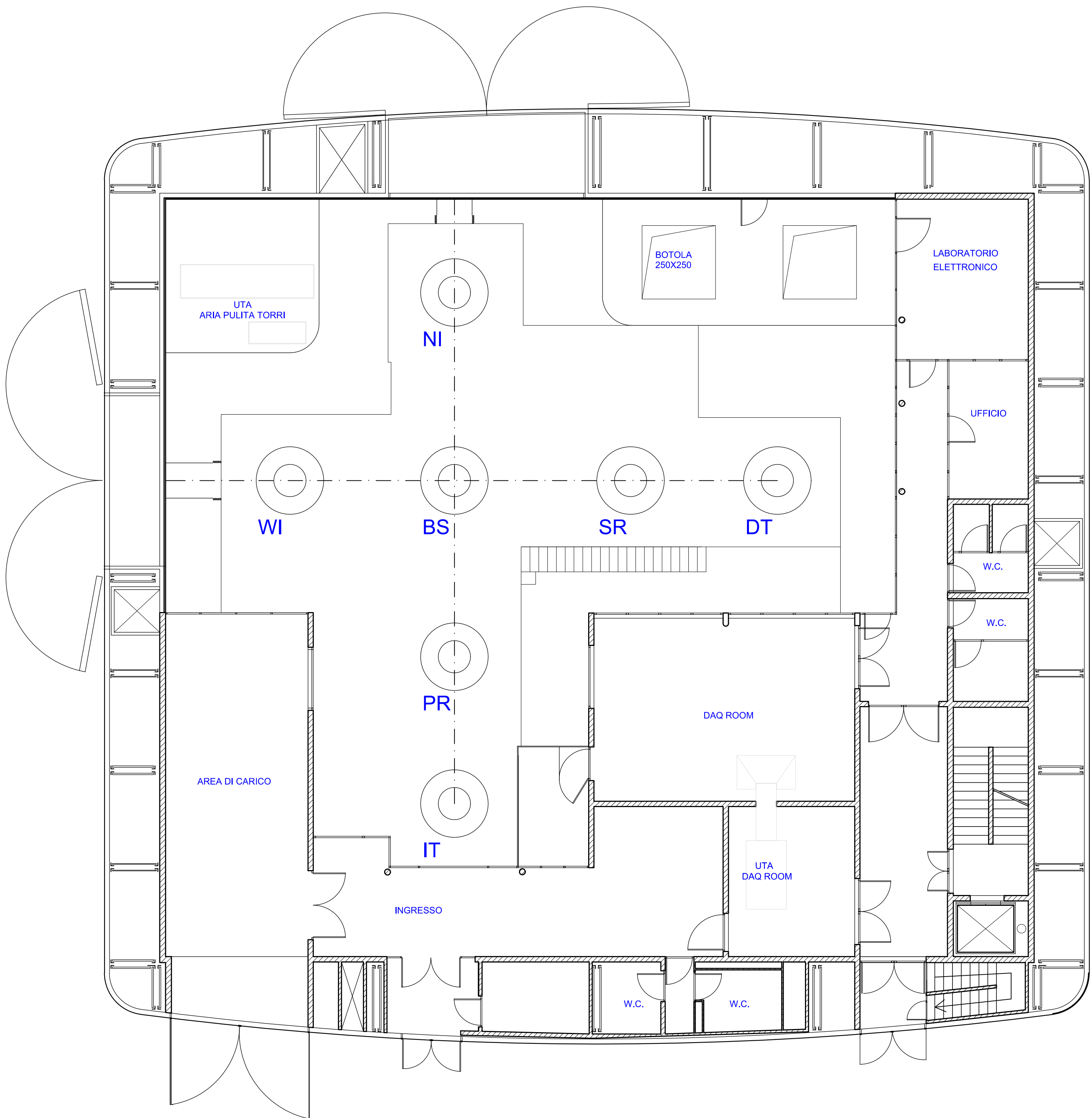
Central Building Level 2 Piano Ingresso
