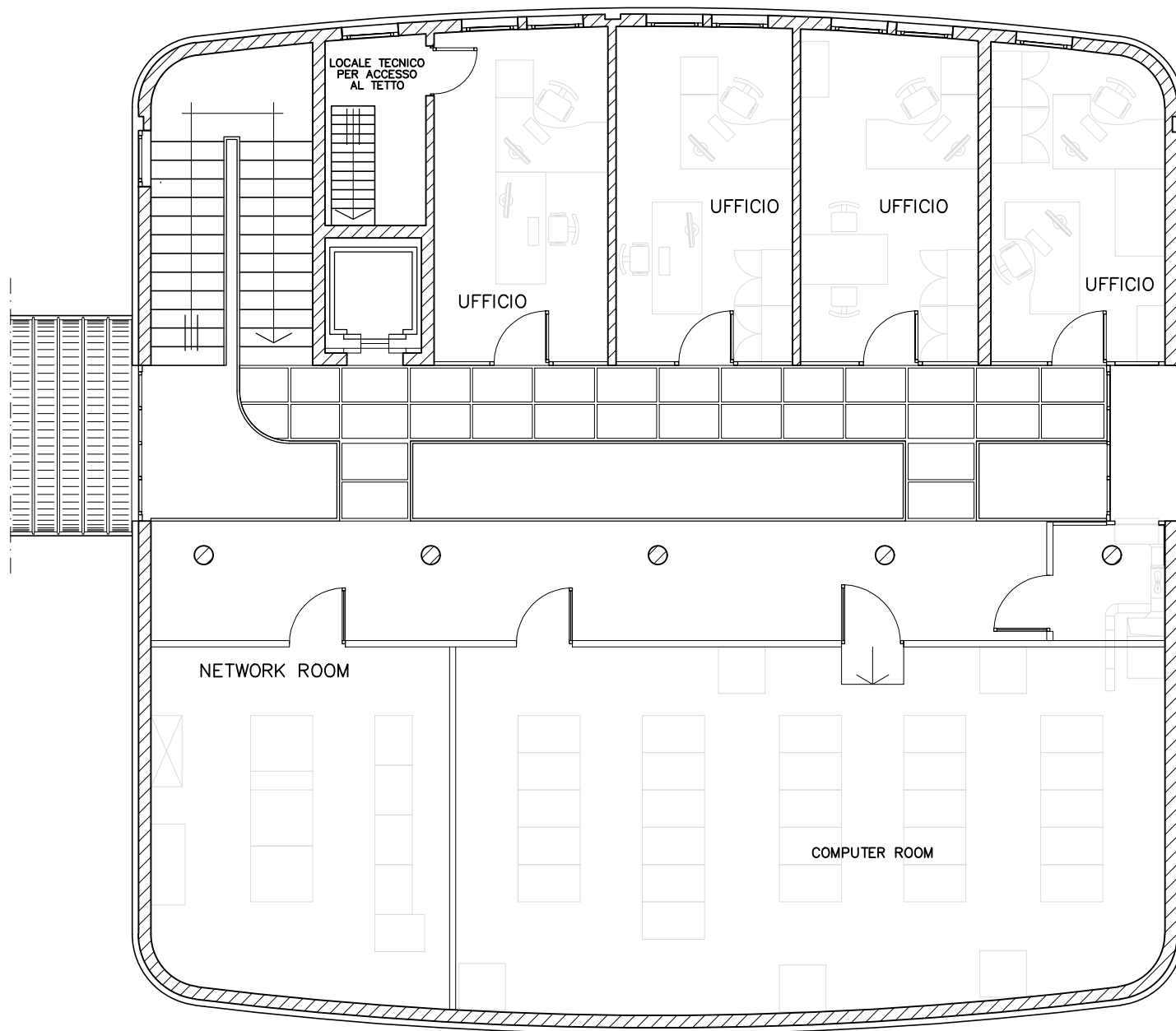
Control Building Piano Primo
